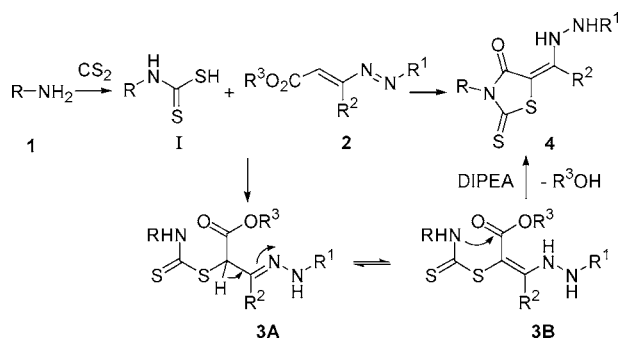
Scheme 2. Plausible Mechanism for the Formation of 5-Hydrazinoalkylidene Rhodanine Derivatives 4
