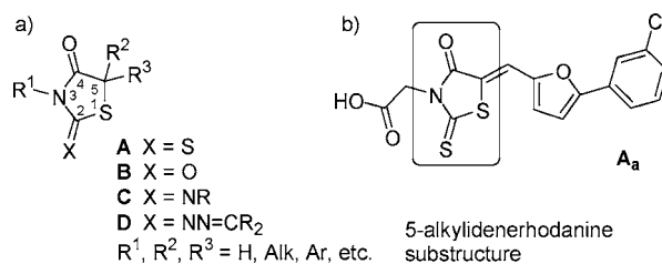
Figure 1. (a) Structures of 4-thiazolidinones. (b) Substituted 5-alkylidene rhodanines A a as an important medicinal structure.
