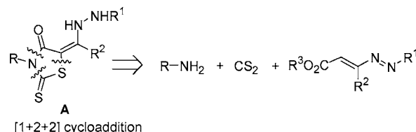
Scheme 1. Retrosynthetic Strategy for the Preparation of 5-Hydrazinoalkylidene Rhodanines
